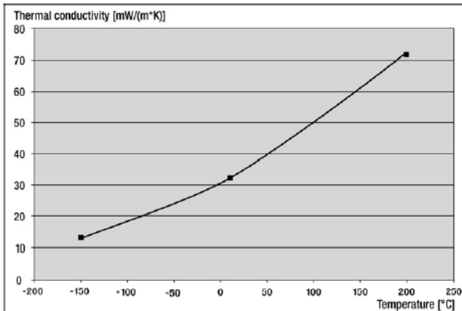
Diagram 2: Thermal conductivity of Basotect® G+. Measurement according to DIN EN 12667 or with the Lola 3 two-plate apparatus manufactured by ZAE Bayem of Würzburg, Germany
