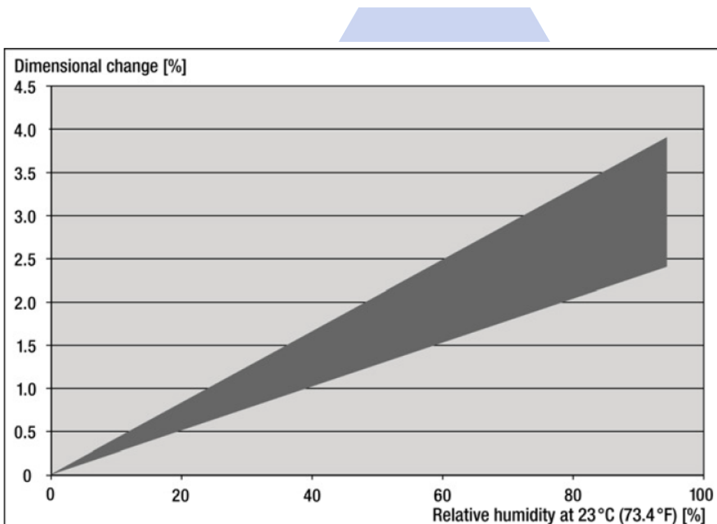
Diagram 1: Dimensional change as a function of the relative indoor humidity at an ambient temperature of 23°C [73.4°F]
